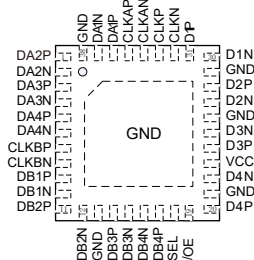
QFN4x4-38L
