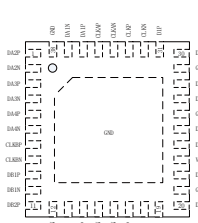
QFN4x4-38L
