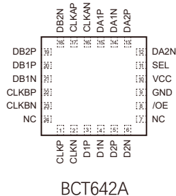
QFN3.4x2.5-24L
