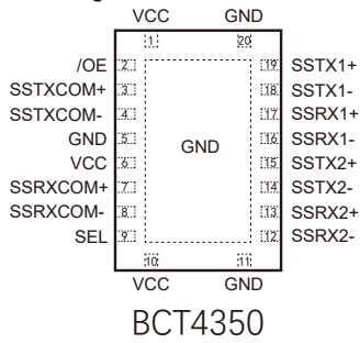
TQFN4.5x2.5-20L
