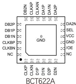
QFN3x3-24L
