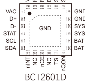
QFN4x4-24L
